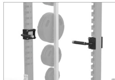
SQUAT HANDLES
